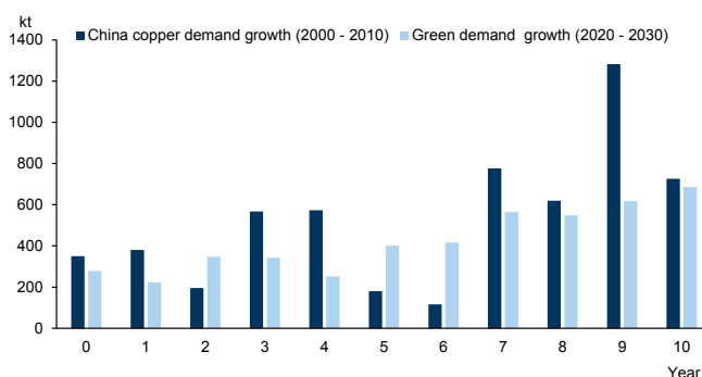
Exhibit 27: Green demand growth volumes will start to surpass previous bull cycle China demand growth from mid-decade China and green copper demand growth
