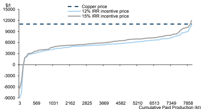
Exhibit 45: Available project data suggests a long-term copper price near $10,000/t is needed to incentivise to enough approvals to mitigate the record LT gap
