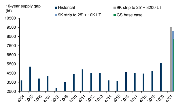
Exhibit 37: Higher price profile modestly reduces the size of the LT supply gap, but sustained high prices key to solving via project approvals
