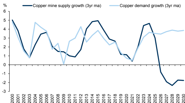
Exhibit 28: Mine copper supply growth decelerates sharply from peak timing in 2024, contrasting with green underpin to demand trend growth
